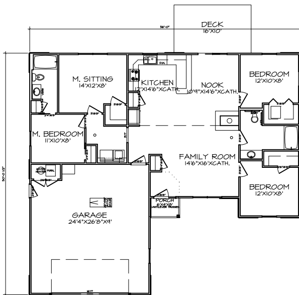
1 FIRST FLOOR PLAN A-4
